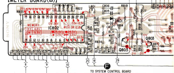
[METER BOARD(B)]
