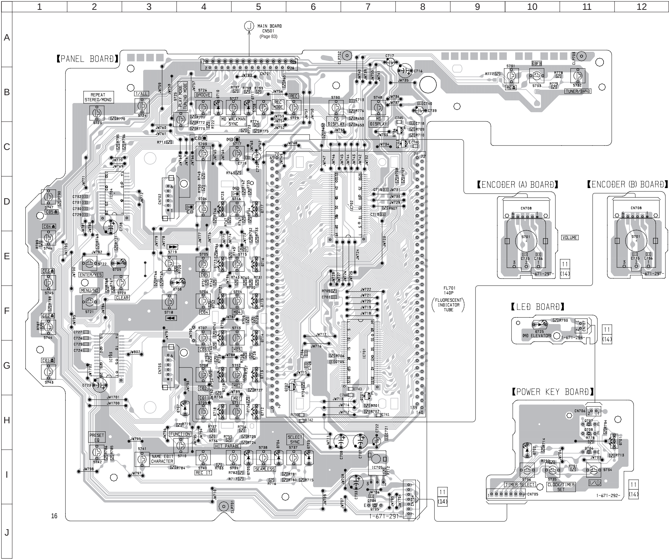
7-21. PRINTED WIRING BOARD — PANEL SECTION — • Refer to page 61 for Circuit Boards Location.
