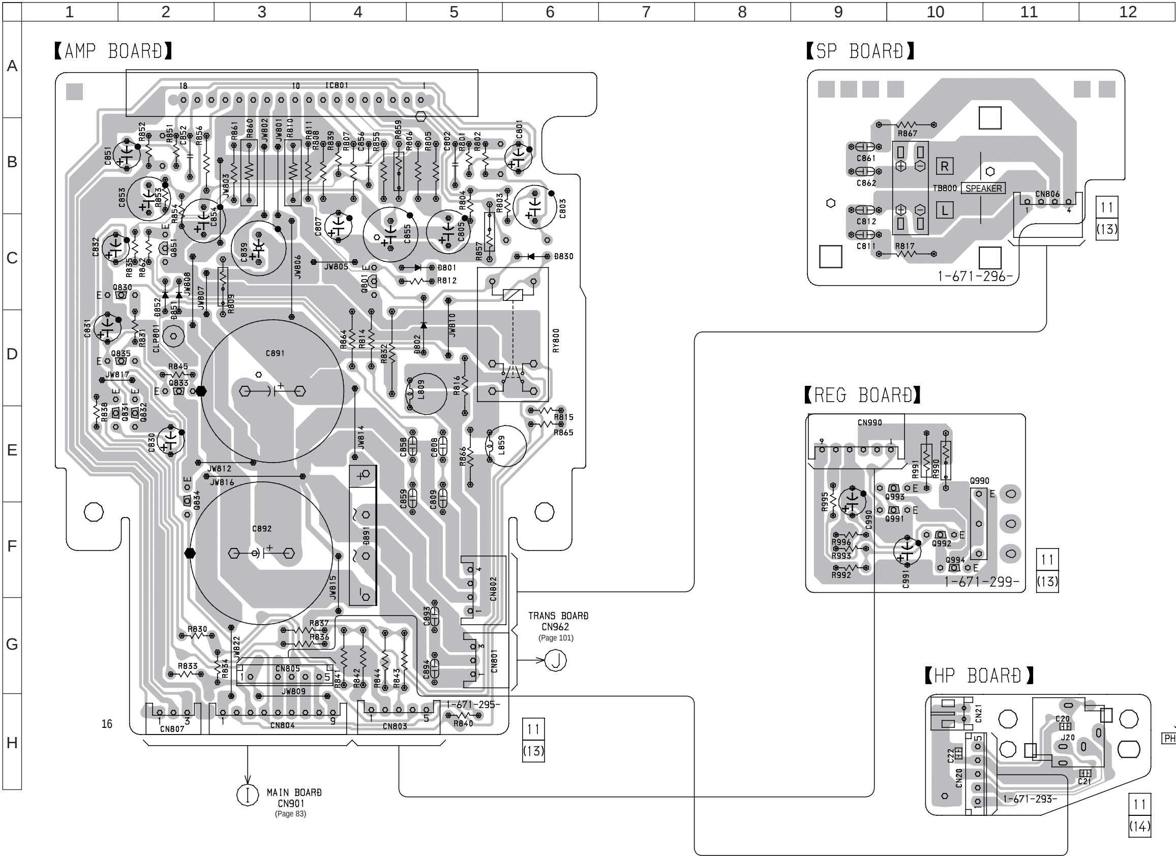
7-19. PRINTED WIRING BOARD — AMP SECTION — • Refer to page 61 for Circuit Boards Location.
