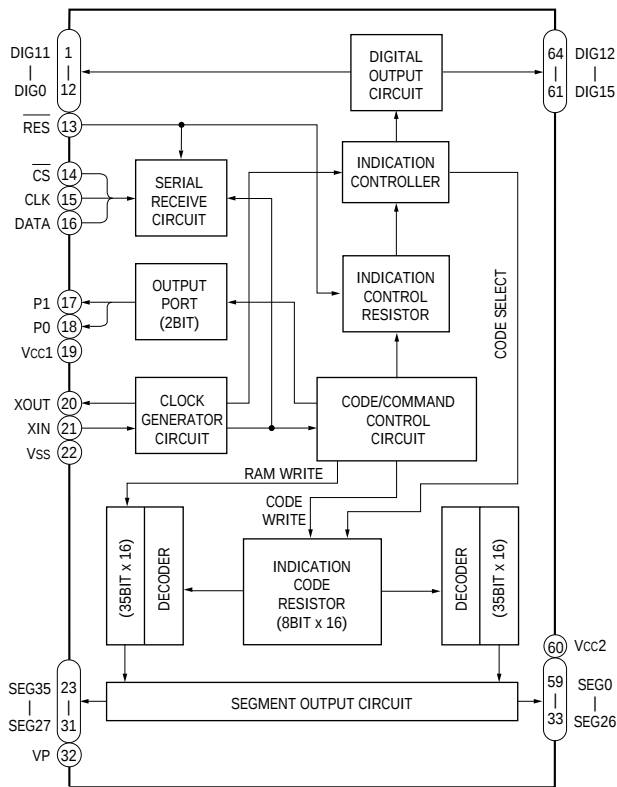
IC701, 702 M66004M8FP
