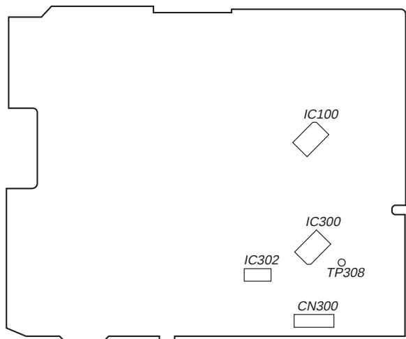
[MAIN Board]
