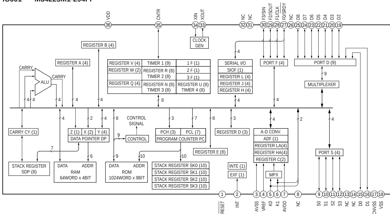
IC601 M34225M1-294FP
