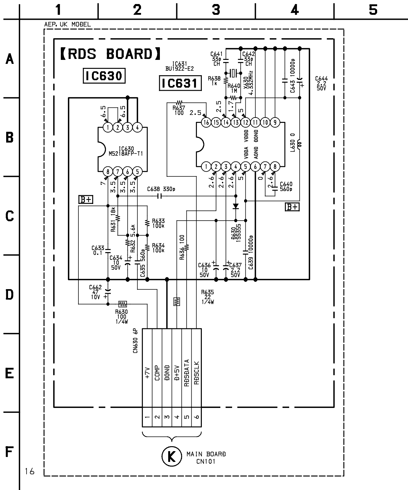
7-10. SCHEMATIC DIAGRAM — RDS SECTION —
