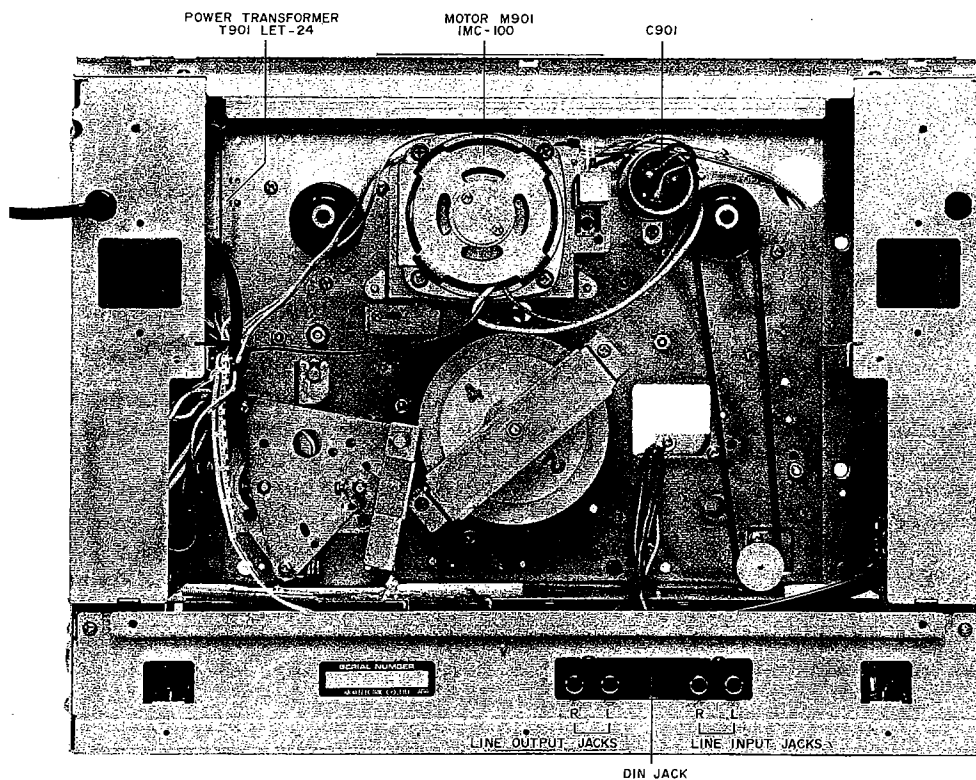
Fig. 3 Rear View (GX-4000D)
