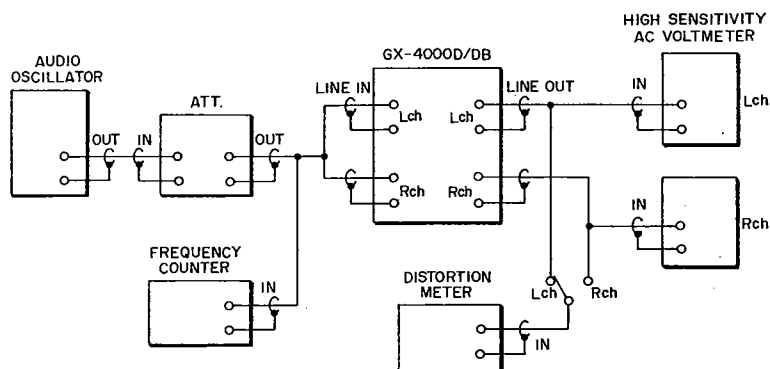
Fig. 11 Instruments Connection
