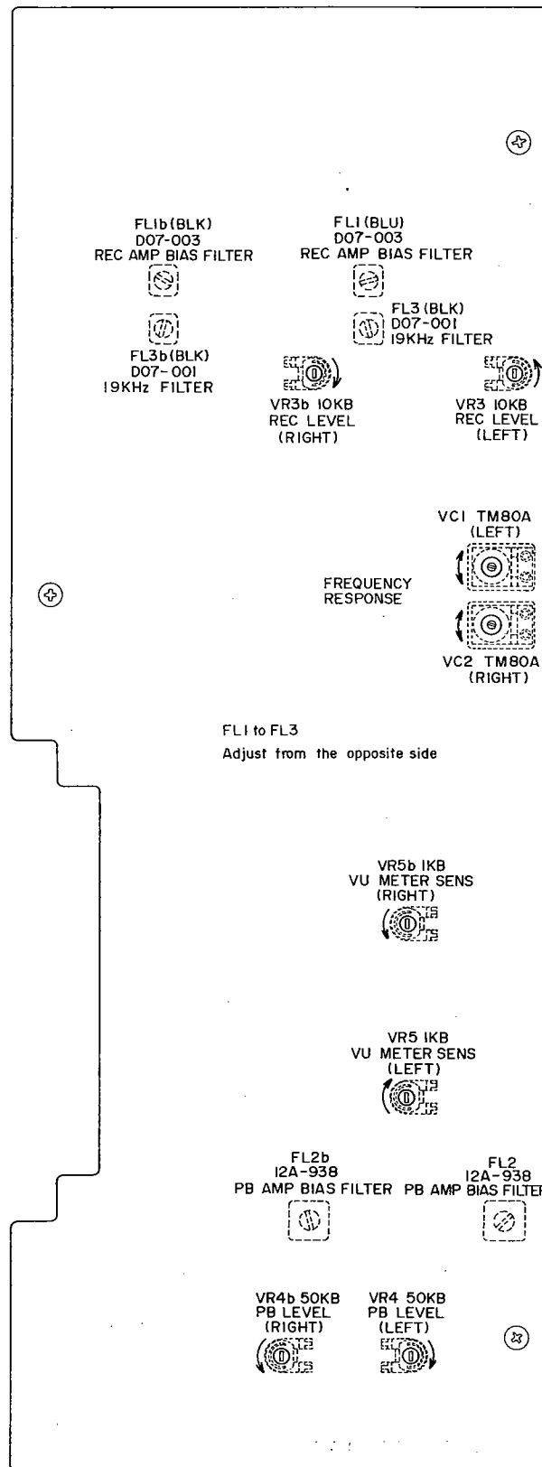
Fig. 13 Amp P.C Board LE-5701A (GX-4000DB)
