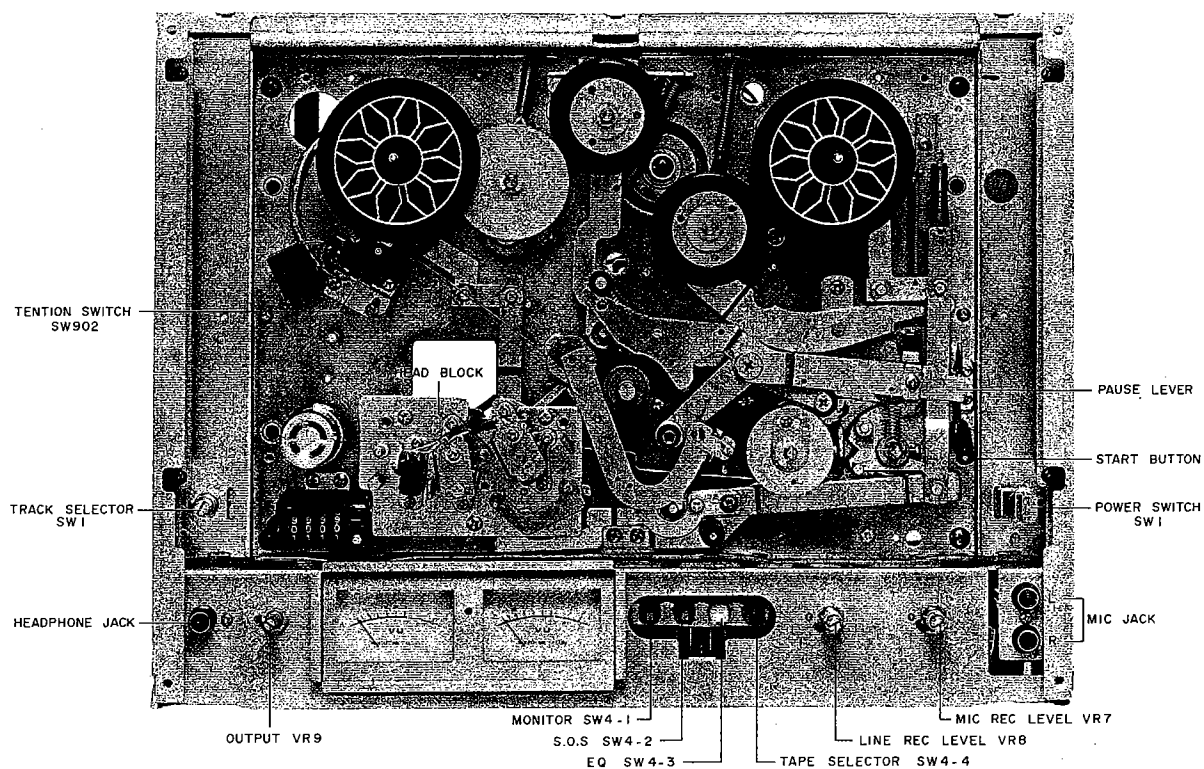
Fig. 2 Front View (GX-4000D)
