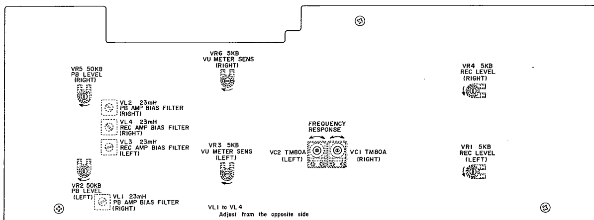
Fig. 12 Amp P.C Board LE-5801A (GX-4000D)
