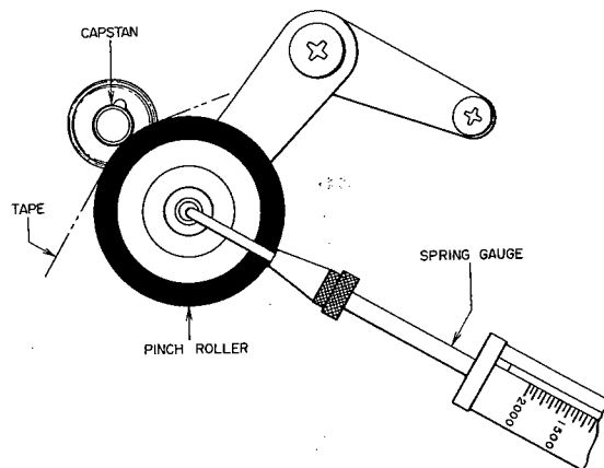
Fig. 4 Pinch Roller Pressure Measurement
